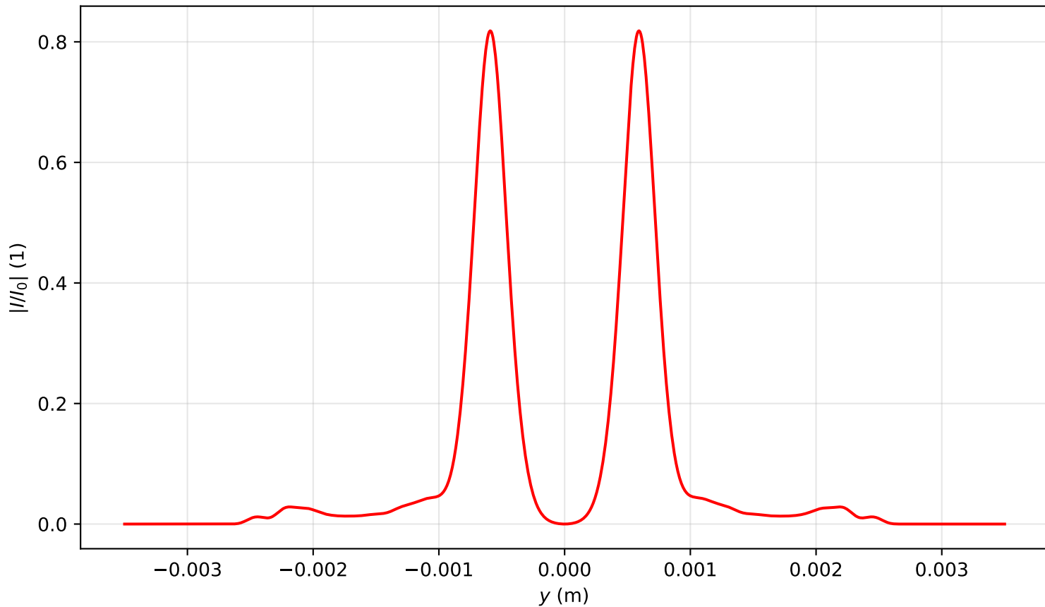
Intensity profile I(x = 0, y, z = 1.990)/I_0 , \text{Pin}=7.0\text{Pcr} , artificial time
